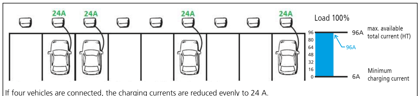
Fig. 11: Example load balancing operating status 2
