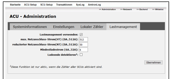
Abb. 13: ACU Administration – Lastmanagement
