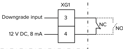
Fig. 13: Schematic circuit diagram: Connection of an external switching contact (default setting: NO)
