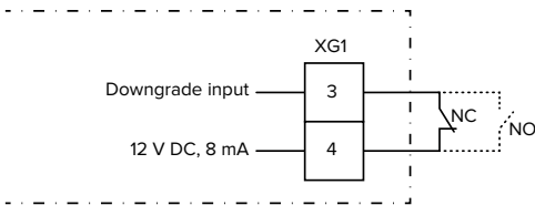
Fig. 13: Schematic circuit diagram: Connection of an external switching contact (default setting: NO)
