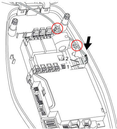
Fig. 14: Enable input connection
