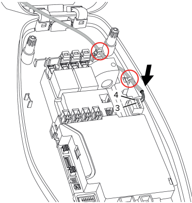
Fig. 12: Tilkobling Downgrade-inngang
