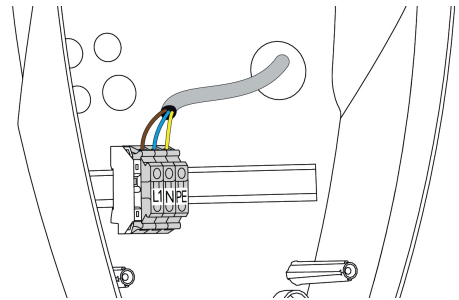
Fig. 8: Power supply connection
