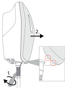
Afb. 4: Frontcover losmaken
