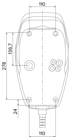
Afb. 6: Boormaten [mm]
