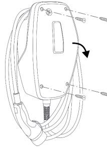
Afb. 5: Product openen
